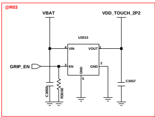
Grip Sensor
